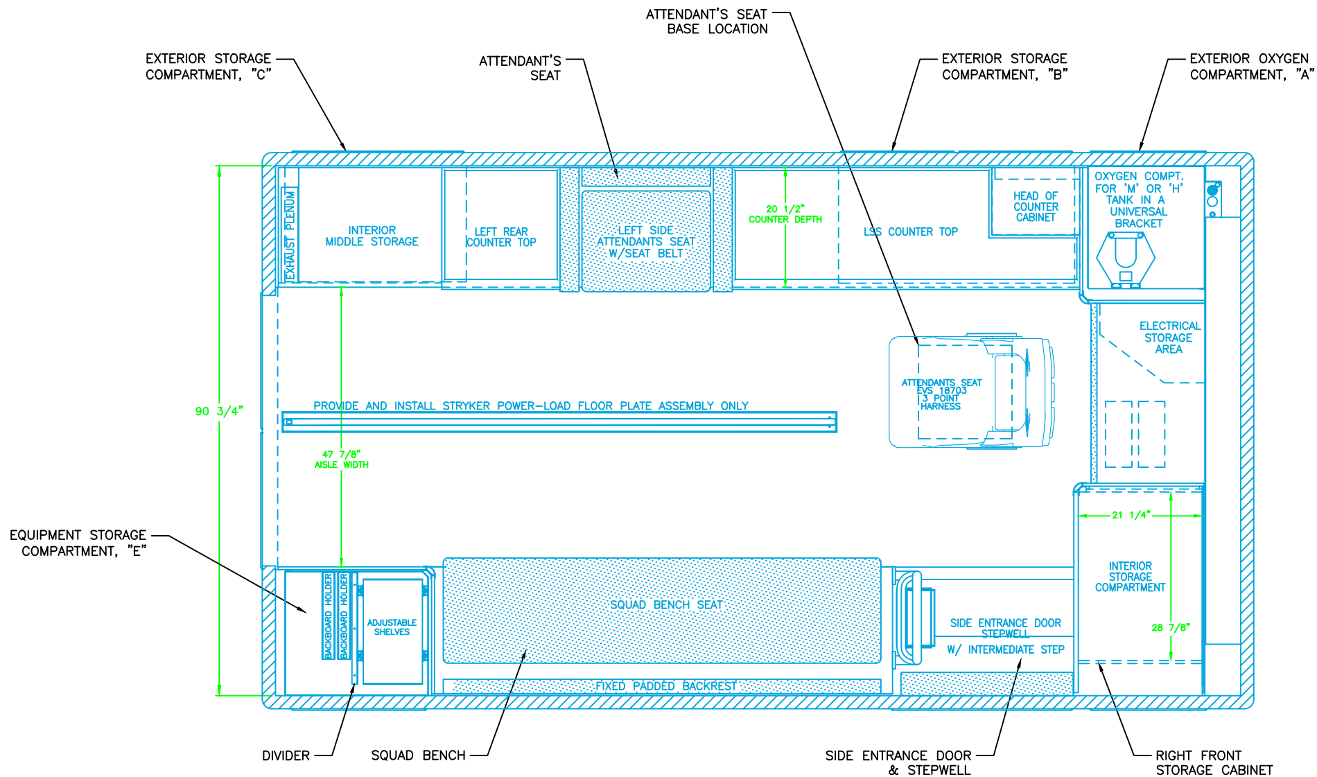
FLOOR PLAN
