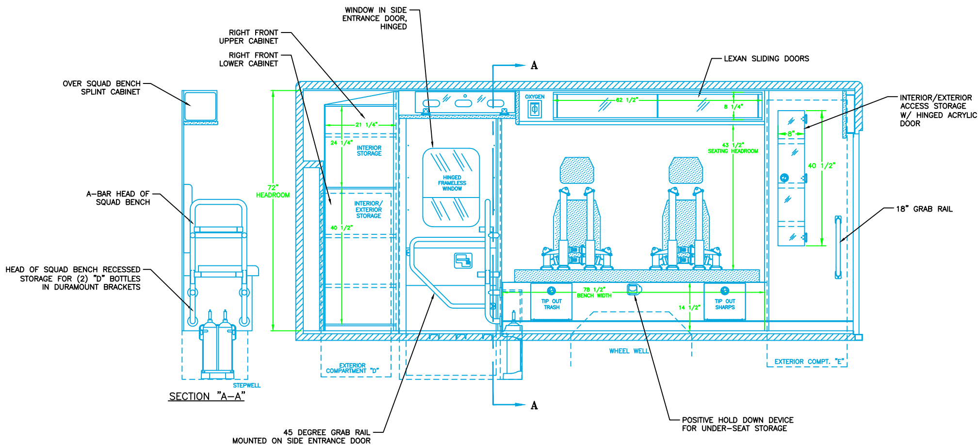
CURBSIDE VIEW
