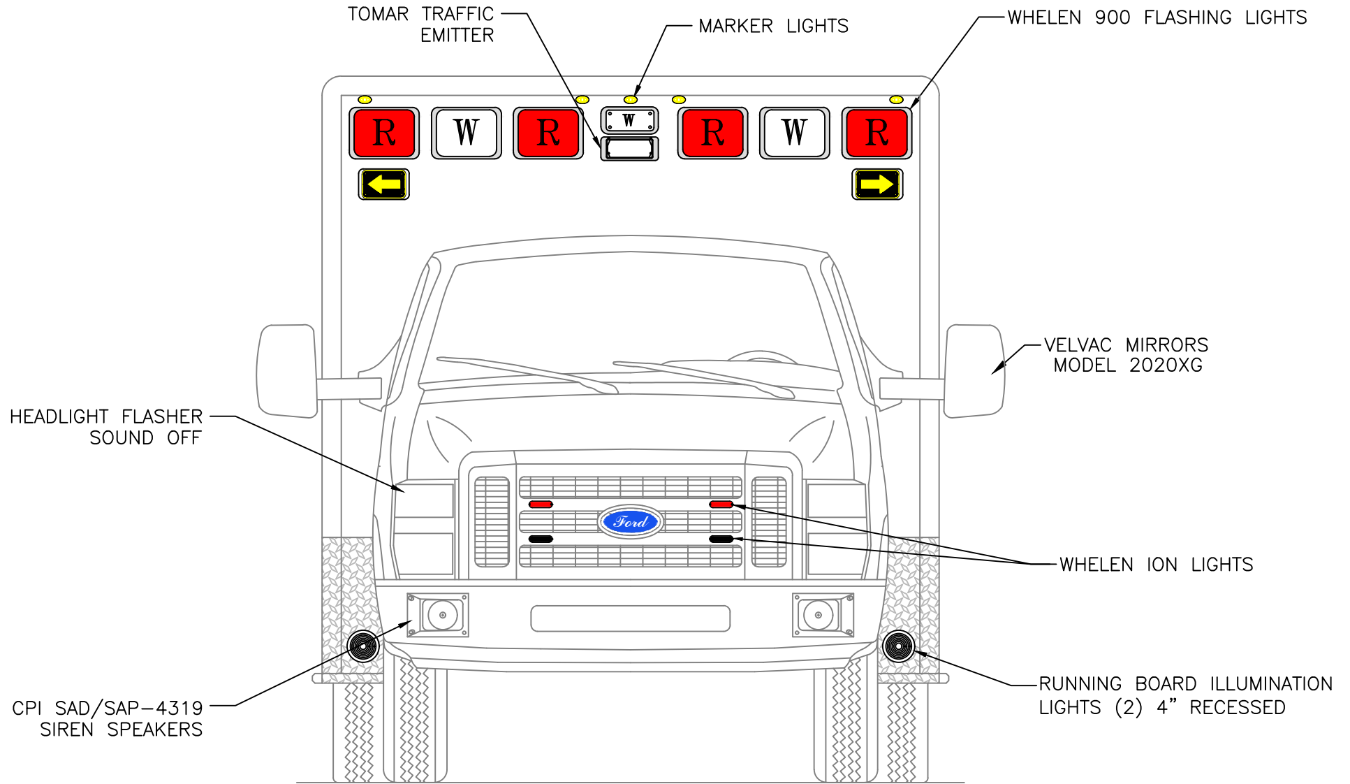
FRONT VIEW
