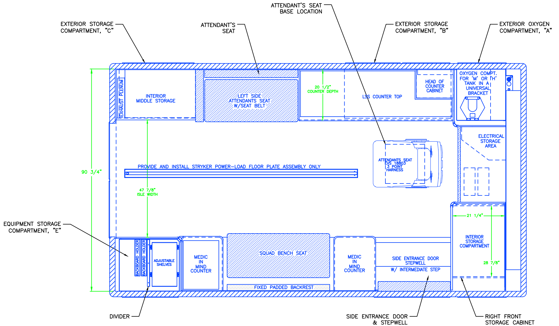
FLOOR PLAN
