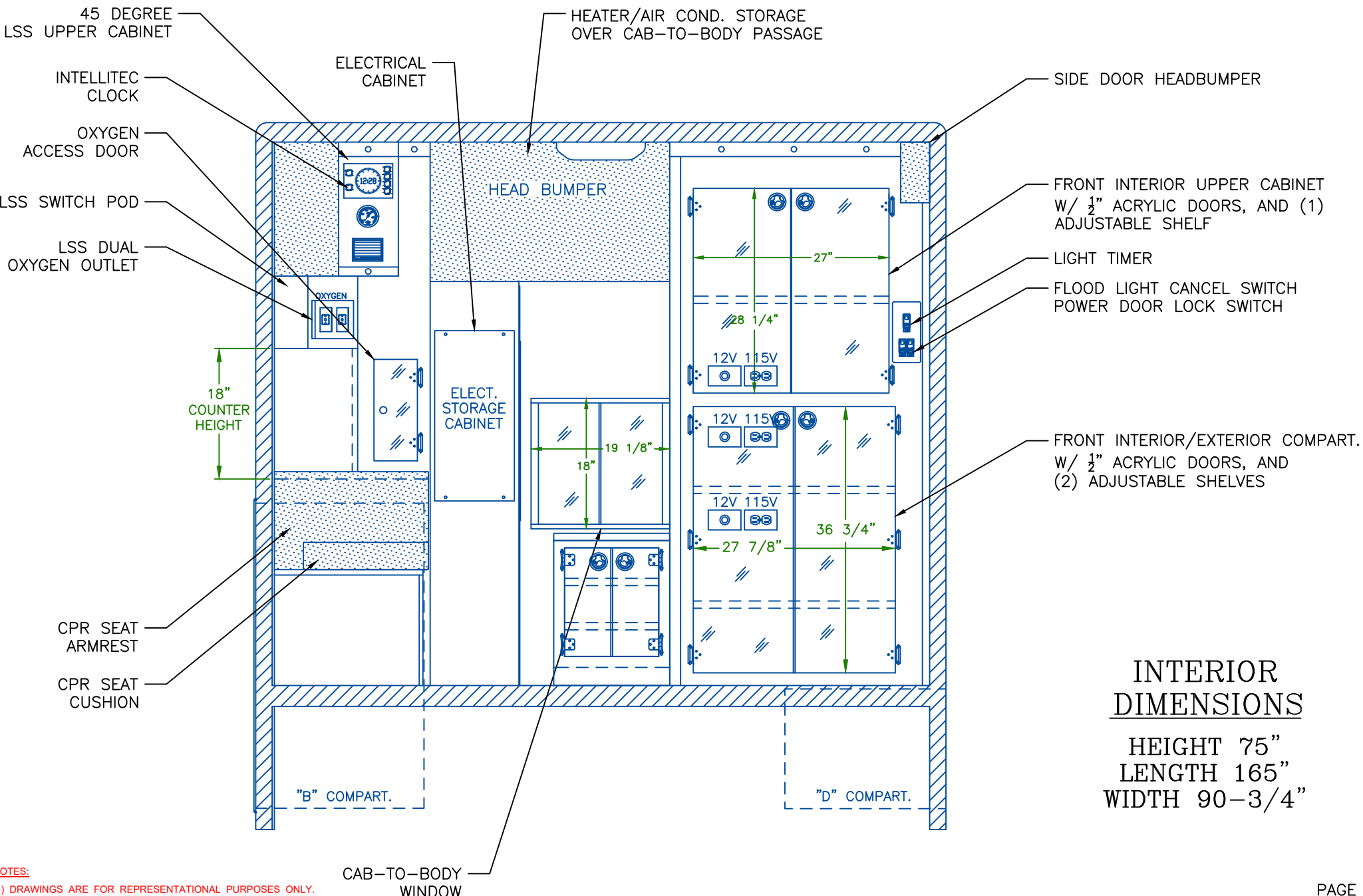
FRONT VIEW
