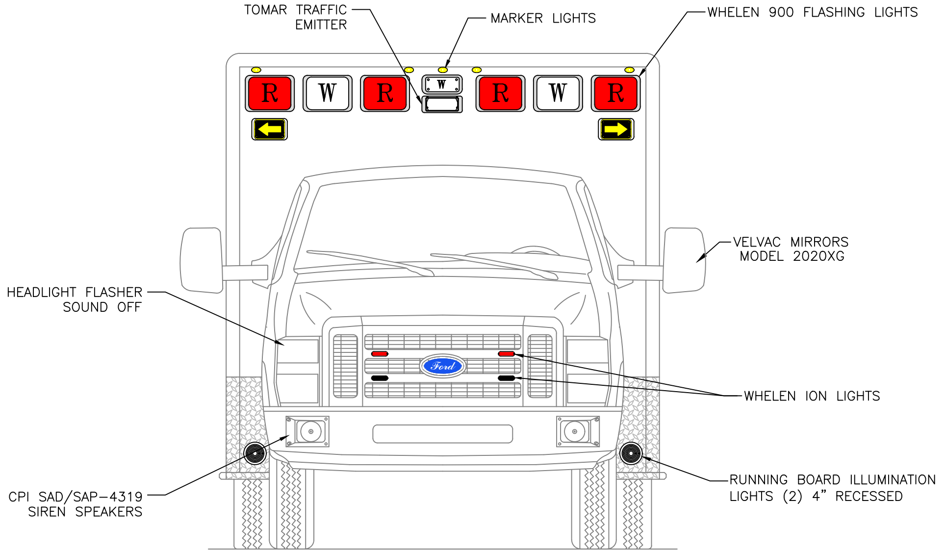
FRONT VIEW
