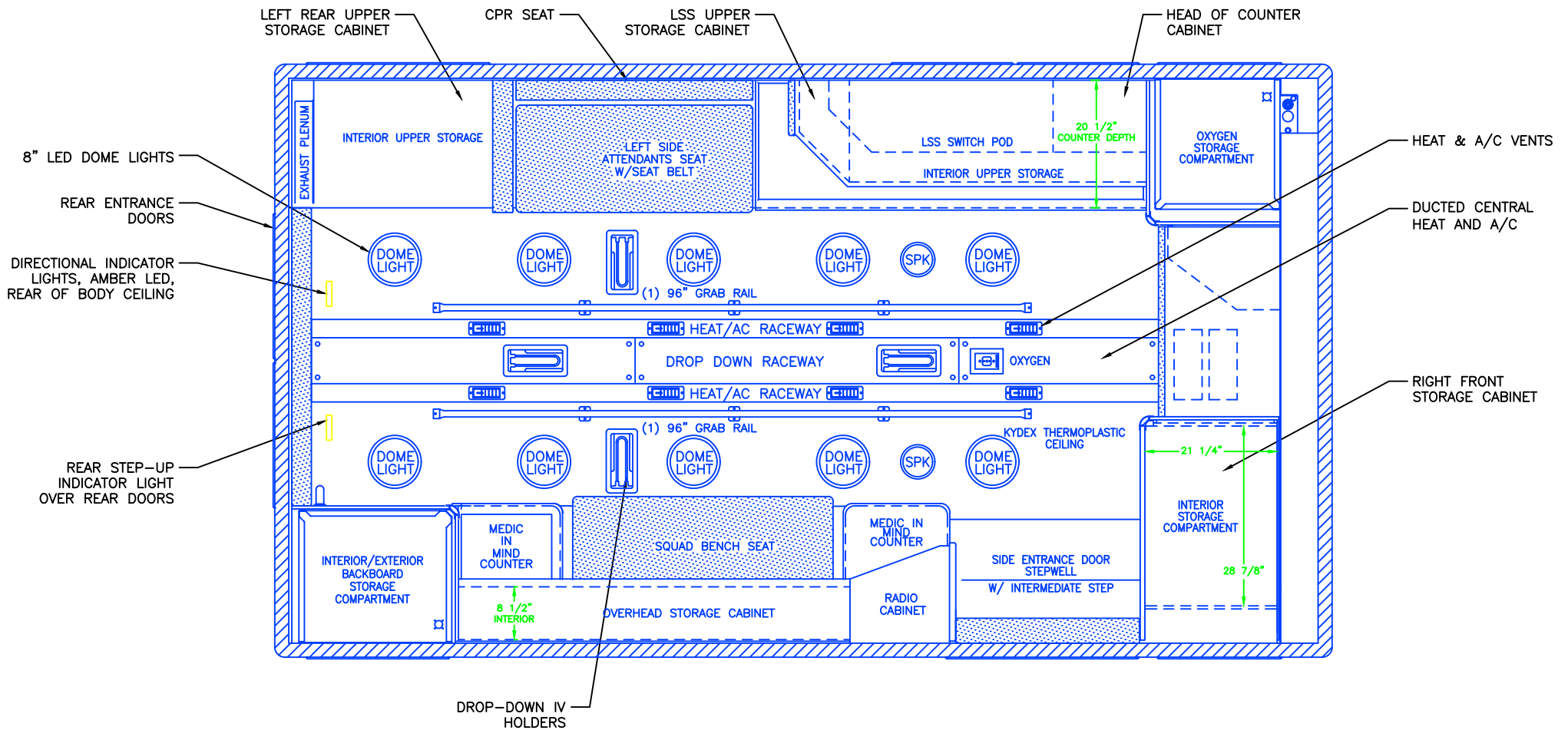
CEILING VIEW
