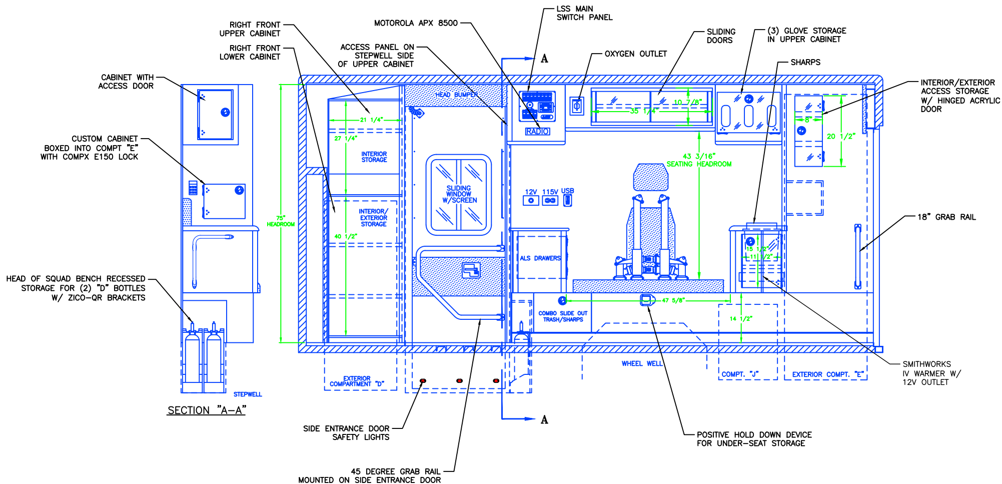
CURBSIDE VIEW
