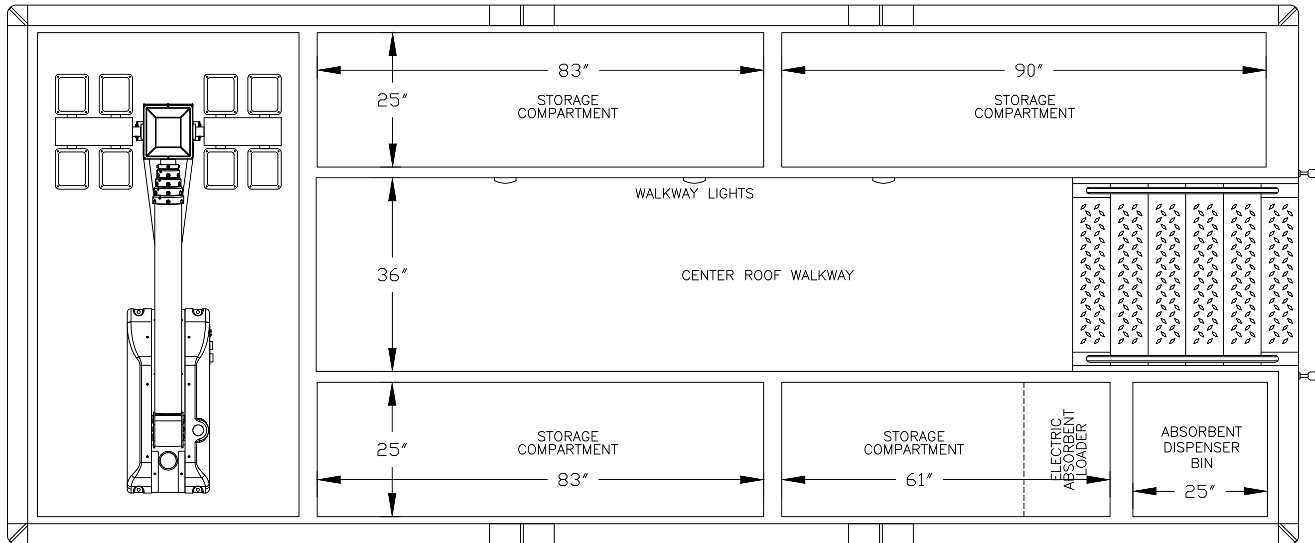
ROOF VIEW
