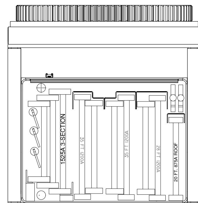
GROUND LADDER ARRANGEMENT
