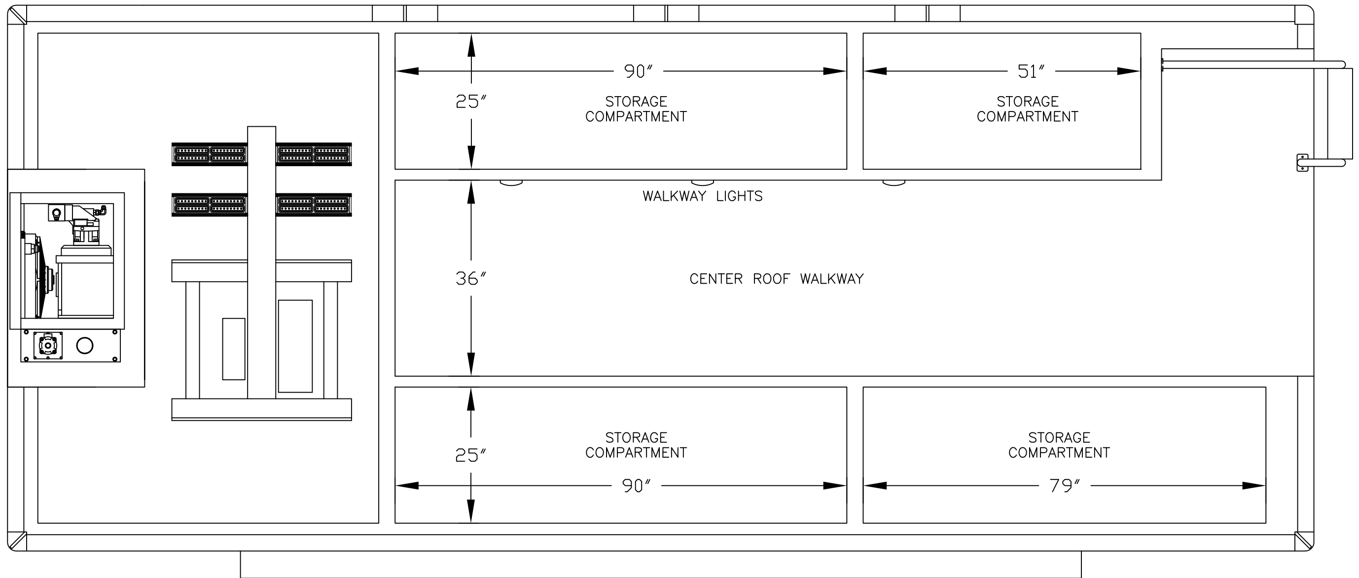
ROOF VIEW
