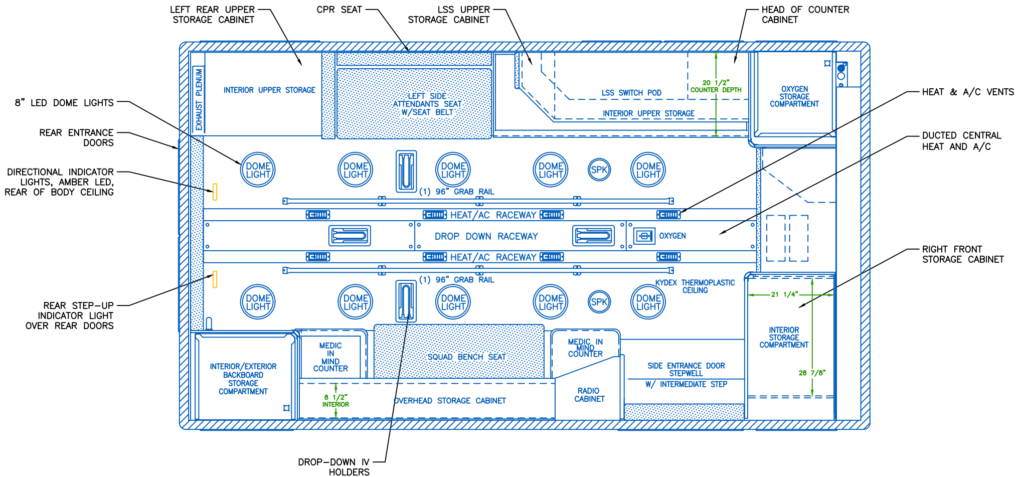
CEILING VIEW
