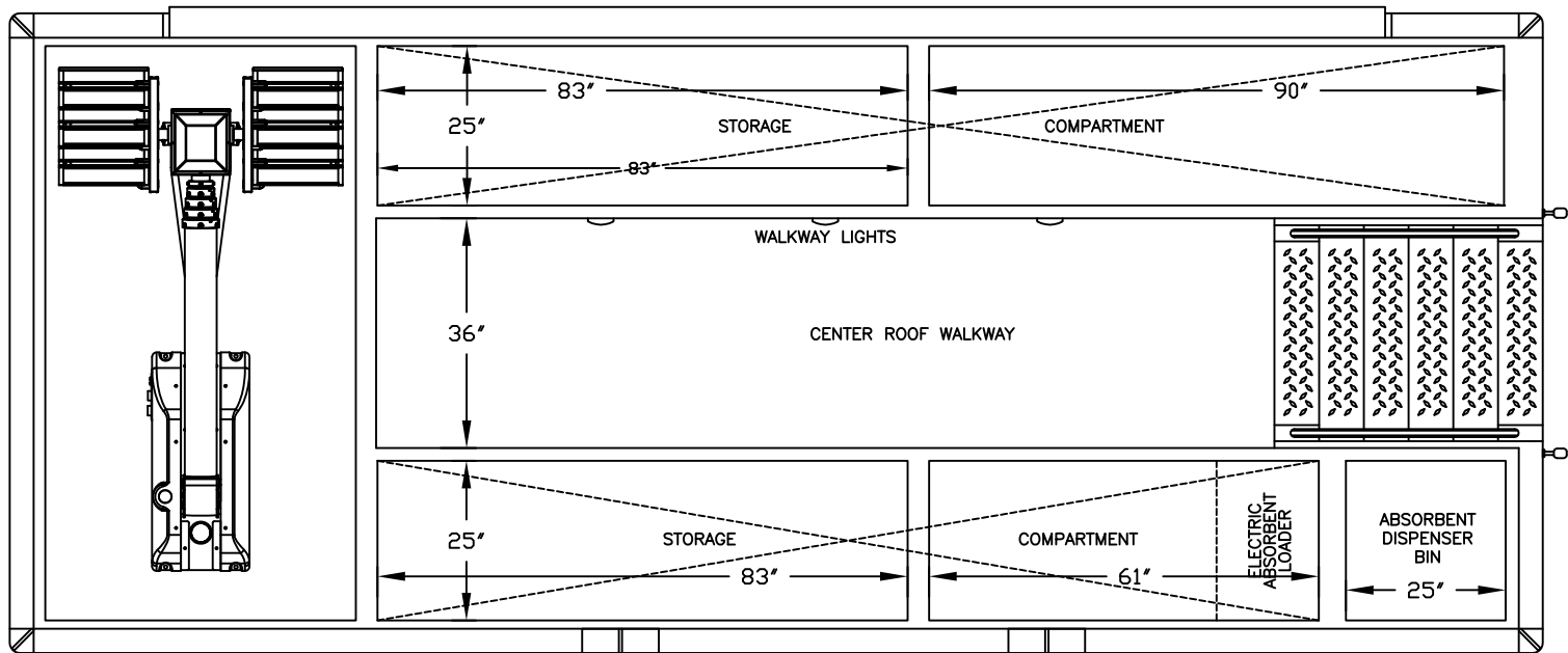
ROOF VIEW
