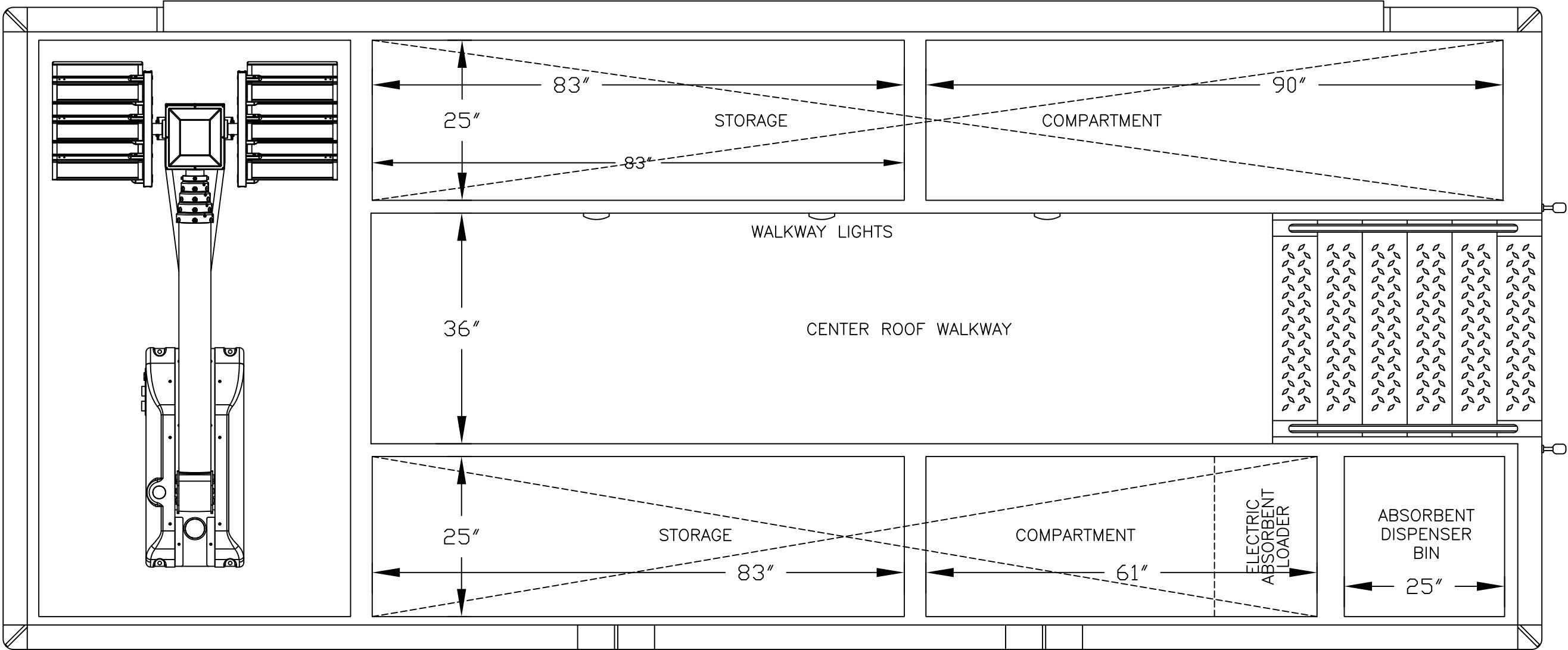
ROOF VIEW
