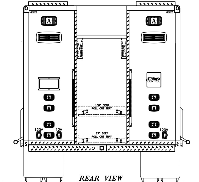
REAR VIEW
